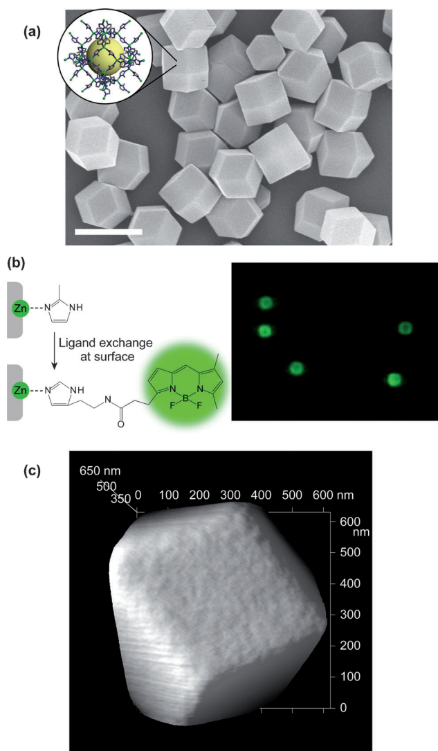
Figure 2. a) Typical SEM image of a dried suspension of original [\text{Zn}(\text{mim})_2]_n particles. Scale bar = 1\ \mu\text{m} . Inset shows the crystal structure of [\text{Zn}(\text{mim})_2]_n . b) Dye modification at the crystal surface and fluorescence image, in liquid suspension, of particles whose surfaces are functionalized with fluorescent dye (excitation at 488 nm). c) AFM image of a typical dye-modified particle.
